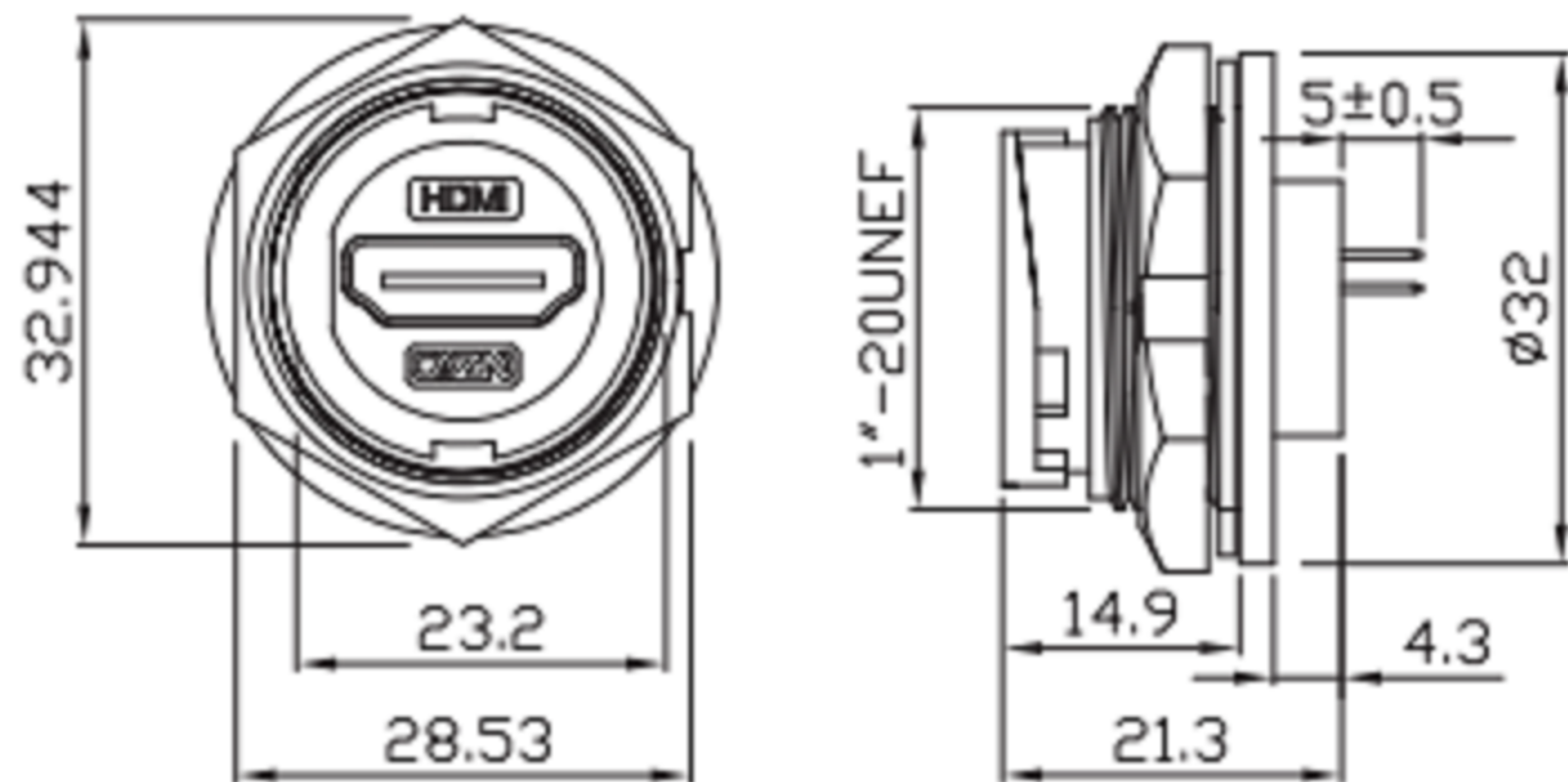
开孔尺寸 hole opening size
